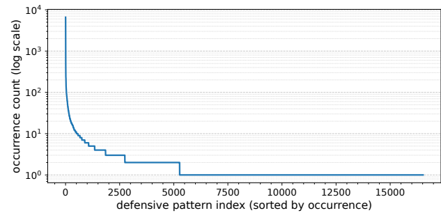
Figure 8: Long-tail occurrences of inferred defensive patterns
