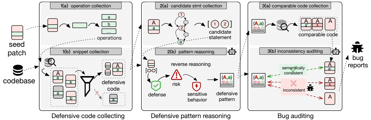
Figure 4: The overall workflow of BugAuditor
